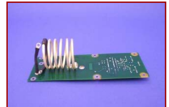
MATCHING NETWORK PERSONALITY (MNP-1) PRO-99-203-001
