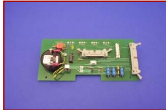
FRONT PANEL INTERFACE (FPI-8) PRO-99-125-008
