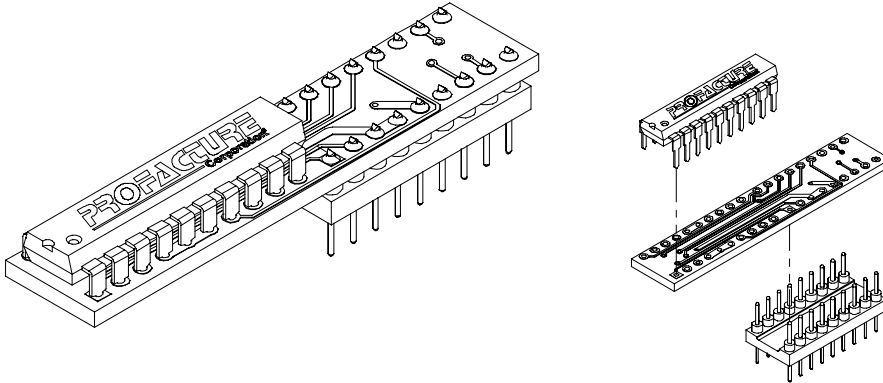
ADAPTER, REPLACEMENT, 4808, SET, U33/U38
