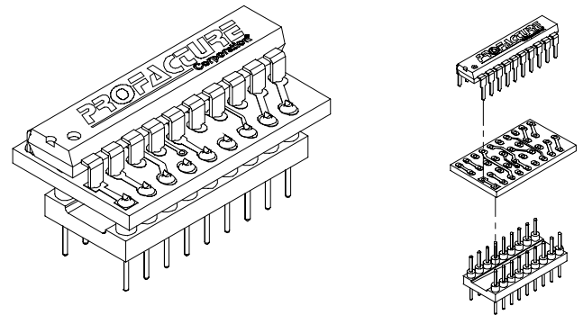
ADAPTER, REPLACEMENT, 4808, SET, U22 - U28
